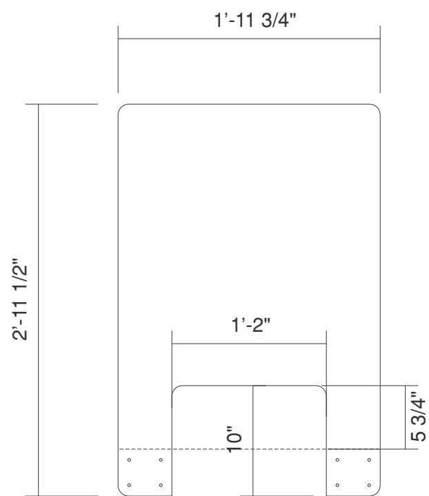
SIZE B 35-1/2" H x 23-3/4" W
