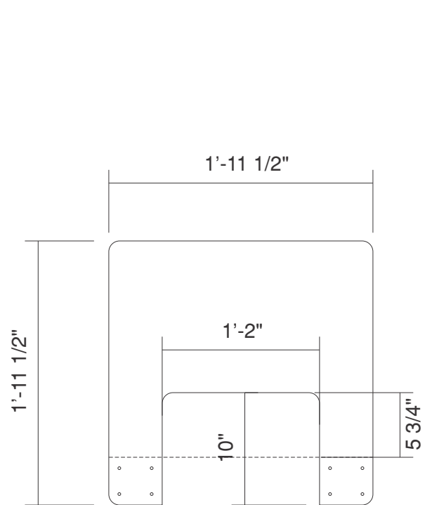
SIZE A 23-1/2" H x 23-1/2" W
