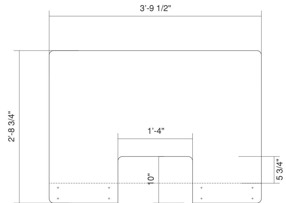
SIZE D 32-3/4" H x 45-1/2" W
