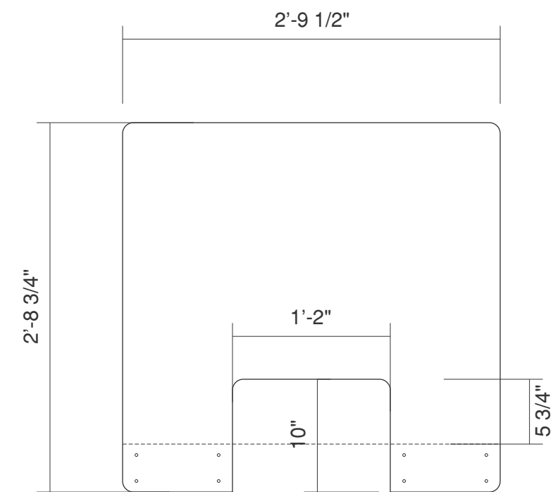
SIZE C 32-3/4" H x 33-1/2" W
